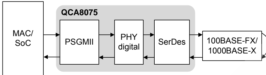
Figure 1-8 External cable loopback, fiber port 4
