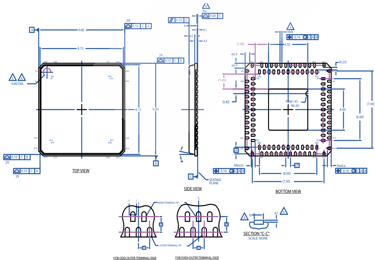
Figure 4-1 QCA8075 mechanical dimensions, top and bottom views (assembly 1)
