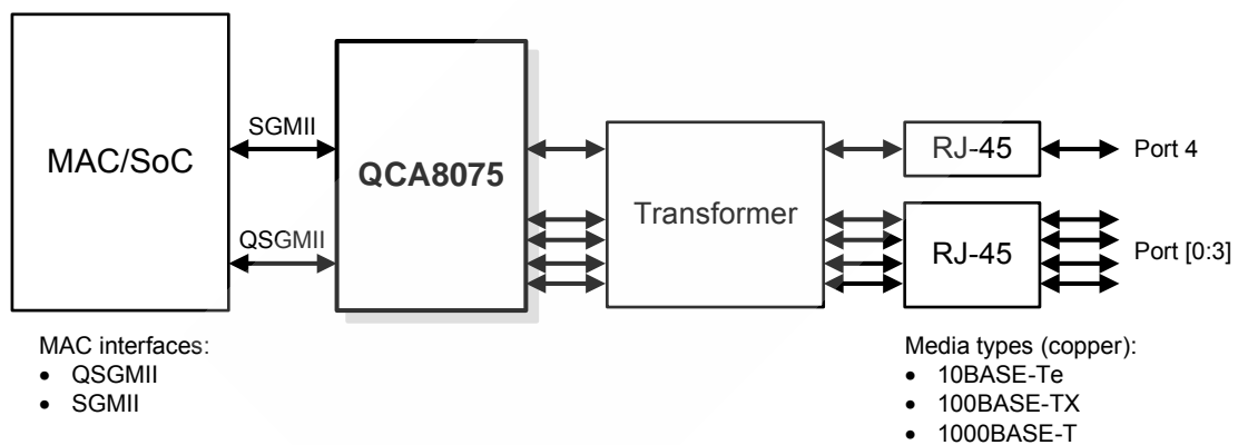
Figure 1-4 QSGMII + SGMII application: 5 copper ports
