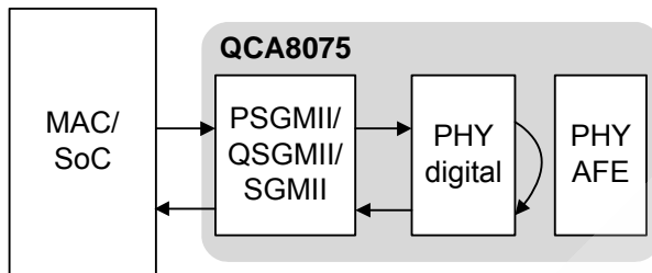
Figure 1-5 Digital loopback, copper port 0 to 4
