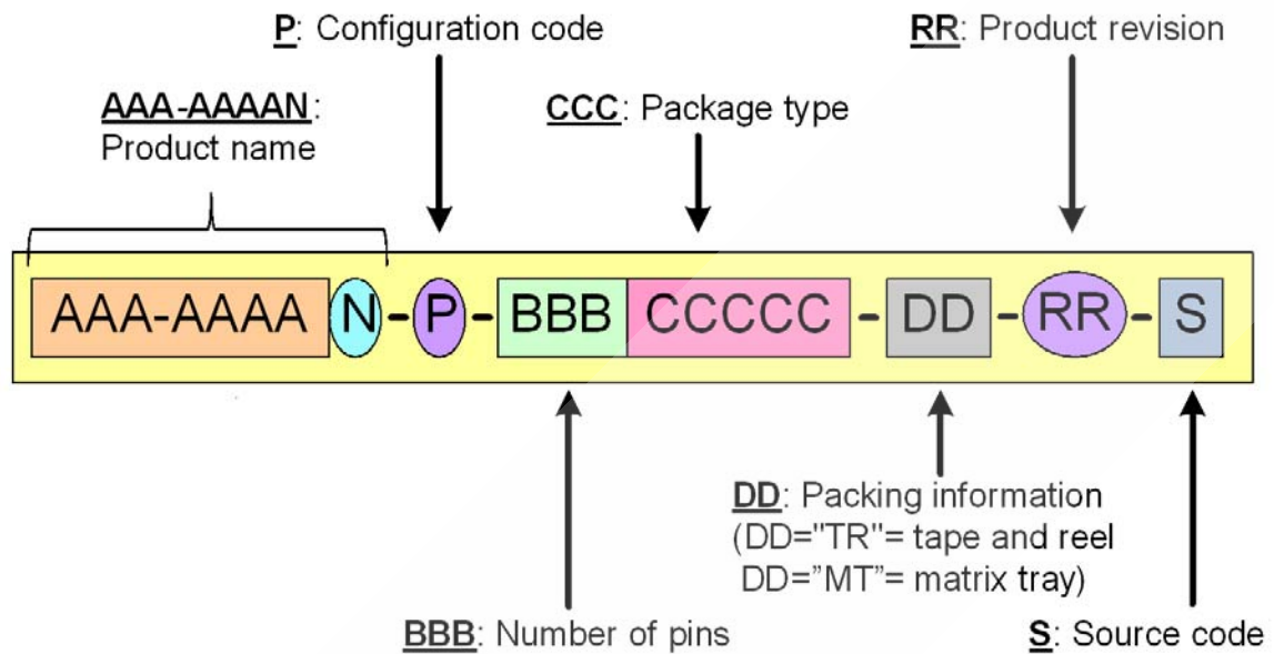
Figure 4-4 Device identification code
